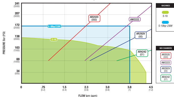
PRESSURE vs FLOW — E-10hp, E-10 with various mix chambers
